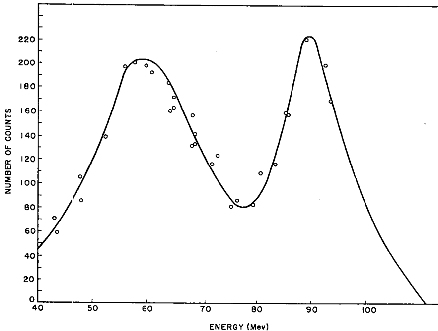
Fig.4 Energy distribution of fission fragments of U^{235} for 2.5-Mev neutrons.
